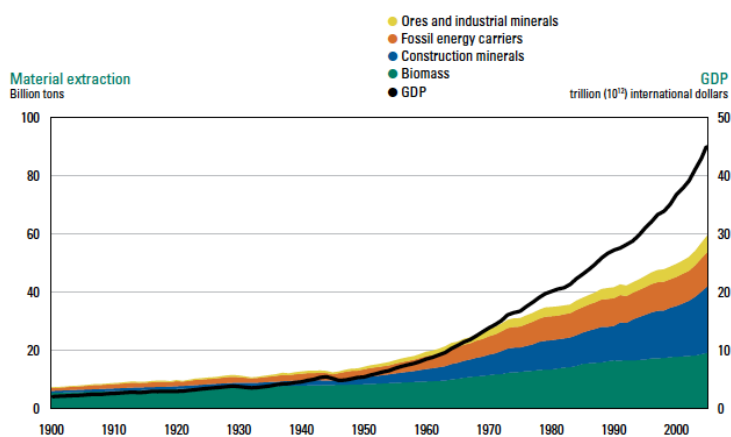
Figure 2. Global material extraction in billion tons, 1900–2005
